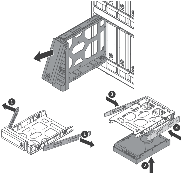
3.5-inch HDD
