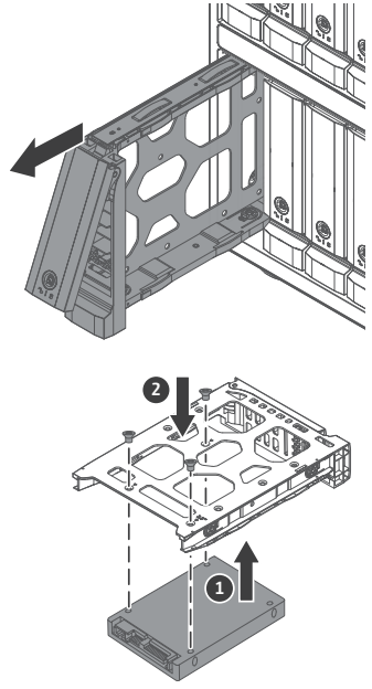
2.5-inch HDD / SSD
