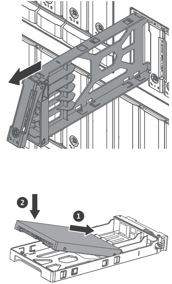
2.5-inch SSD
