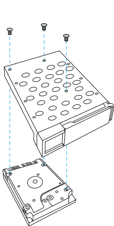
2.5" HDD/SSD
